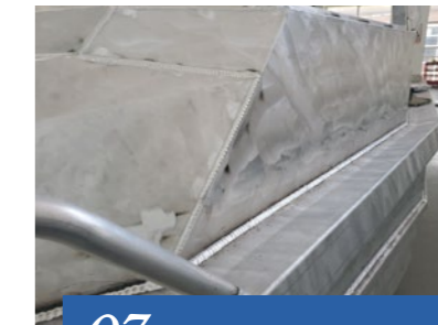
07 Welding details
